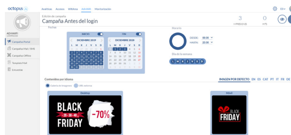
Image 4. Campaign customization.
